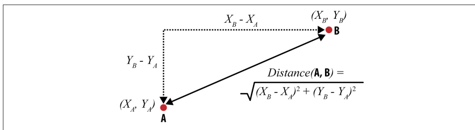
Figure 6-1. Euclidean distance.
